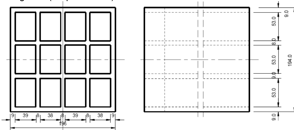
Figure 3 (Brique Creuse)
