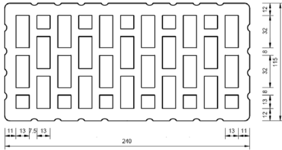
Figure 1 (HLz)
